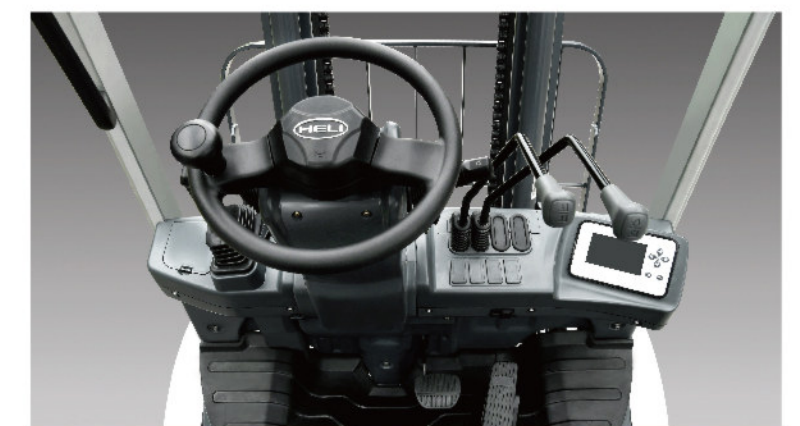
IC truck type control valve stem, better fit to the driver's habits
